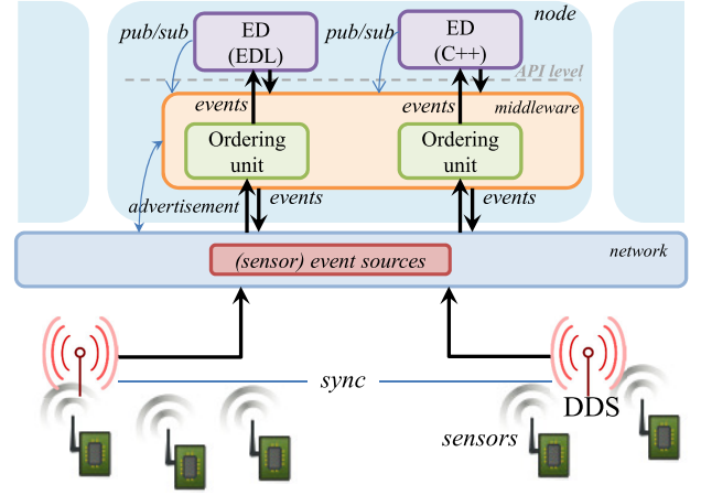
Fig. 2. Distributed publish/subscribe EBS.
