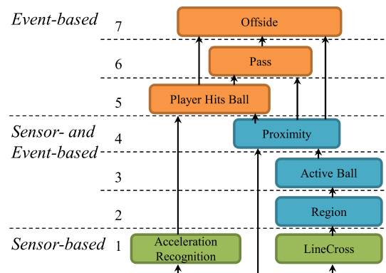
Fig. 1. Event hierarchy for an offside rule violation.
