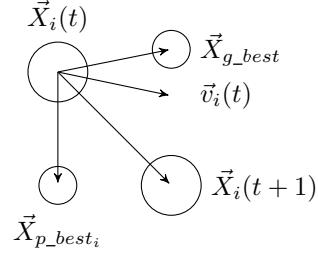
Fig. 3. The way PSO combines weighted forces.
