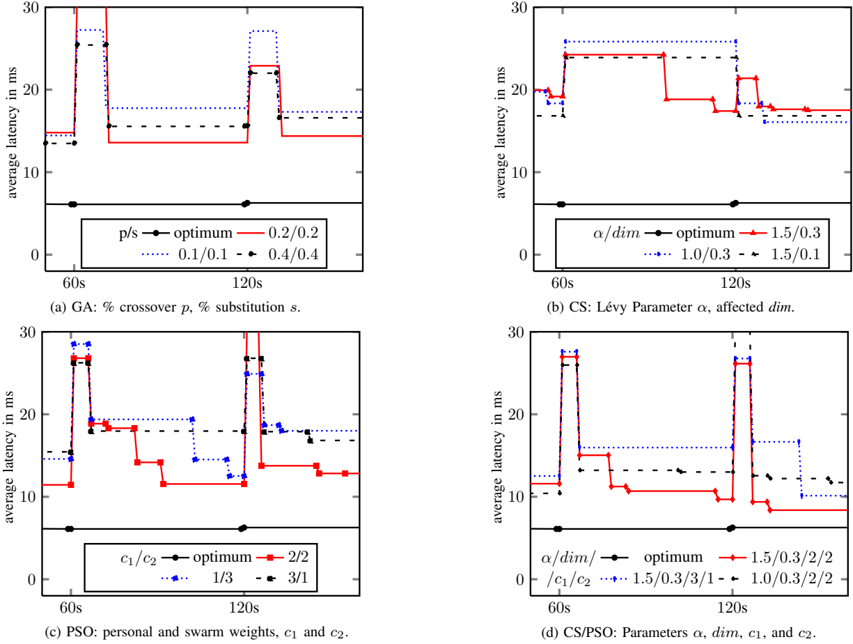
Fig. 6. Dynamic latency adaption achieved by GA, CS, PSO and CS/PSO.
