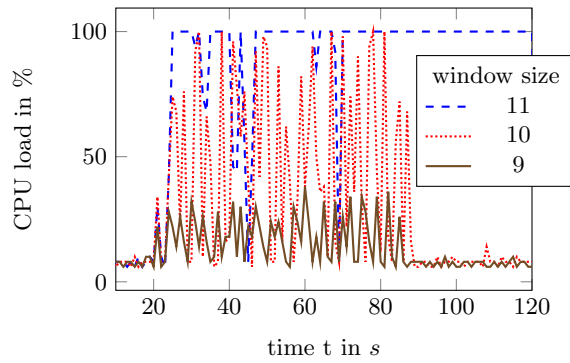
Figure 7: System loads for different window sizes.
