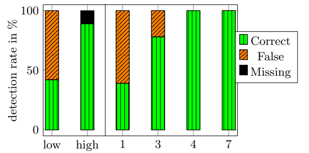
left: baseline CEP, low/high detection thresholds right: approximative CEP, various sliding window sizes
