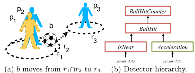
Figure 1: Uncertainty in event detection.
