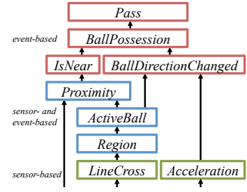
Figure 5: Benchmark event detection hierarchy.
